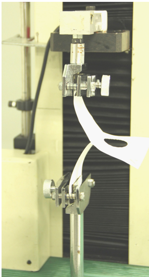
Fig. 5 – Tensile strength test. The two ends of the stapled paper were pulled by a testing machine and the tensile force that could open the anastomosis was registered.
